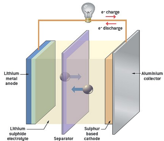
Fig1. The Chemistry of Li-S extracted from OXIS Energy
