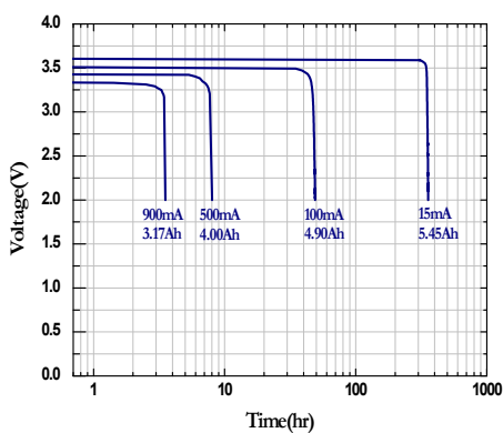
Continuous Discharge at 20°C
