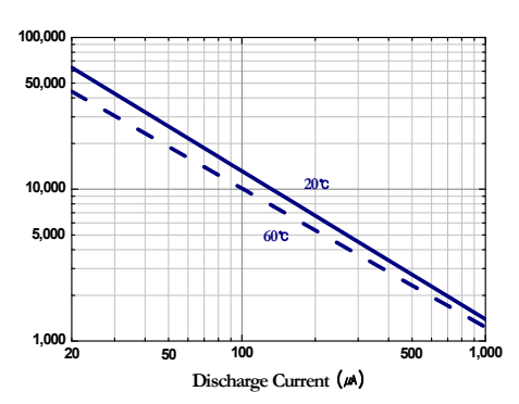
Discharge Current vs. Duration Time
